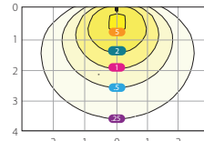
Photometric Report #X34-100LSF-U DLF1907101-2A C.I.E.S
