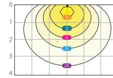
Photometric Report #X34-155LSF-U DLF1907101-4A C.I.E.S
