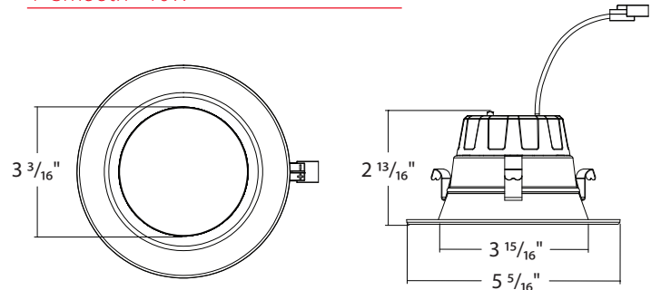
4" Smooth - 10W
