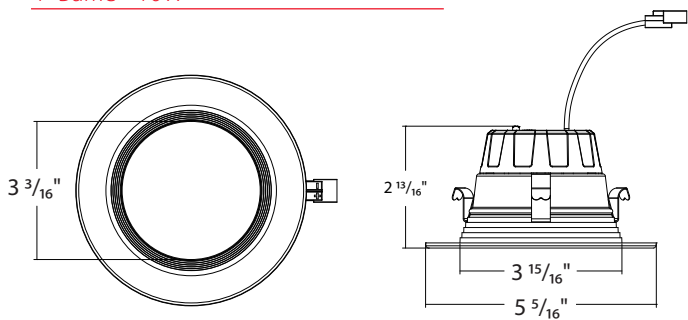
4" Baffle - 10W
