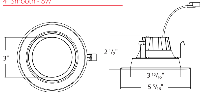
4" Smooth - 8W
