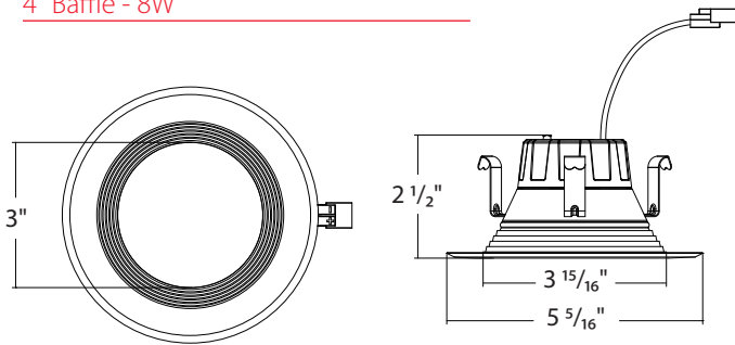
4" Baffle - 8W
