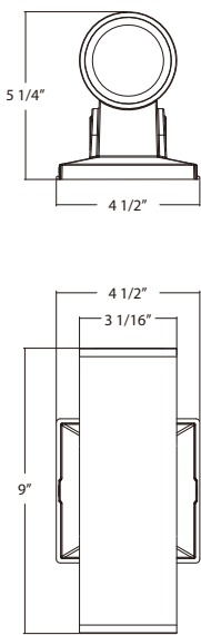
3" Wall Mount Weight: 2.67lbs
