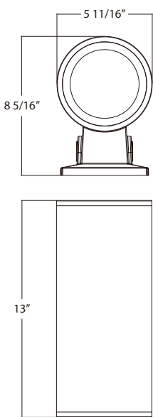
6" Wall Mount Weight: 6.35 lbs
