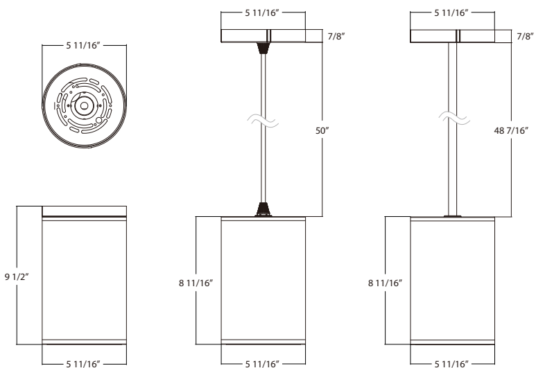
6" Surface, Cord, Pendant Weight: 4.34 lbs
