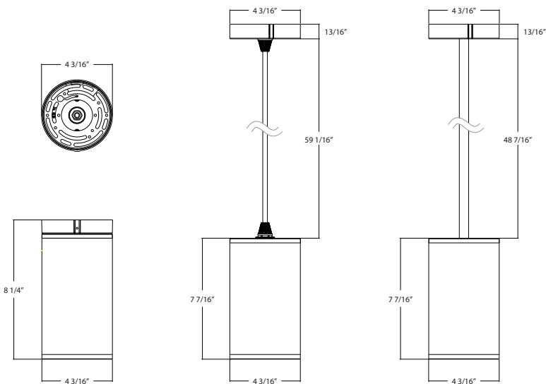
4" Surface, Cord, Pendant Weight: 2.68 lbs
