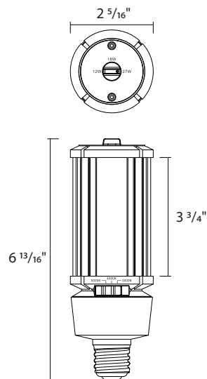
HIDFA27S E26 Base
