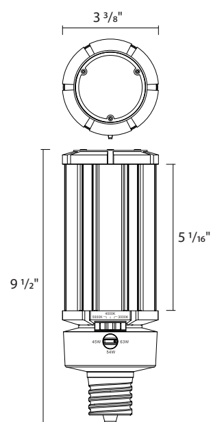
HIDFA63S EX39 Base
