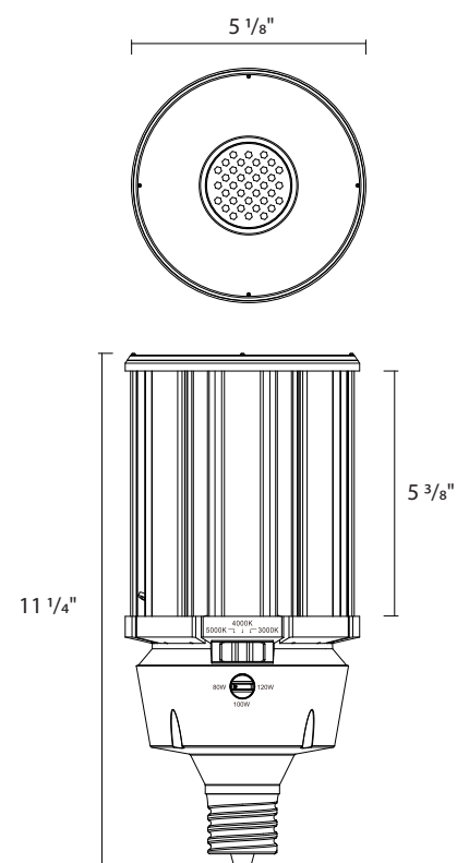
HIDFA120S EX39 Base
