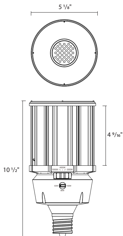
HIDFA100S EX39 Base
