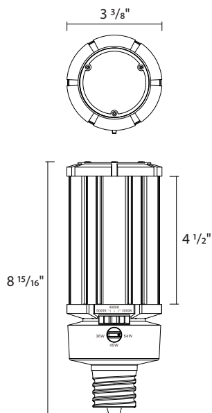
HIDFA54S EX39 Base
