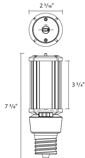
HIDFA27S EX39 Base
