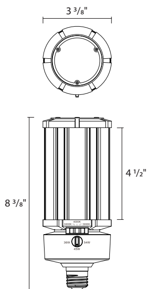
HIDFA54S E26 Base
