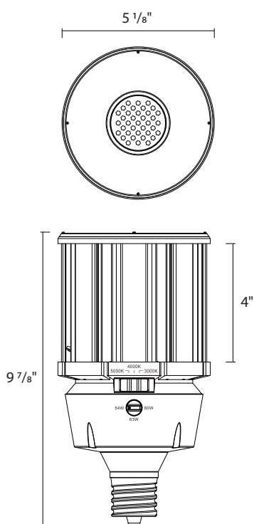
HIDFA80S EX39 Base
