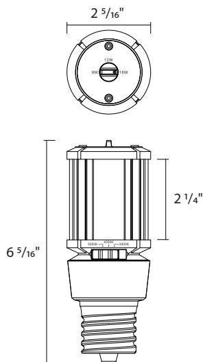
HIDFA18S EX39 Base
