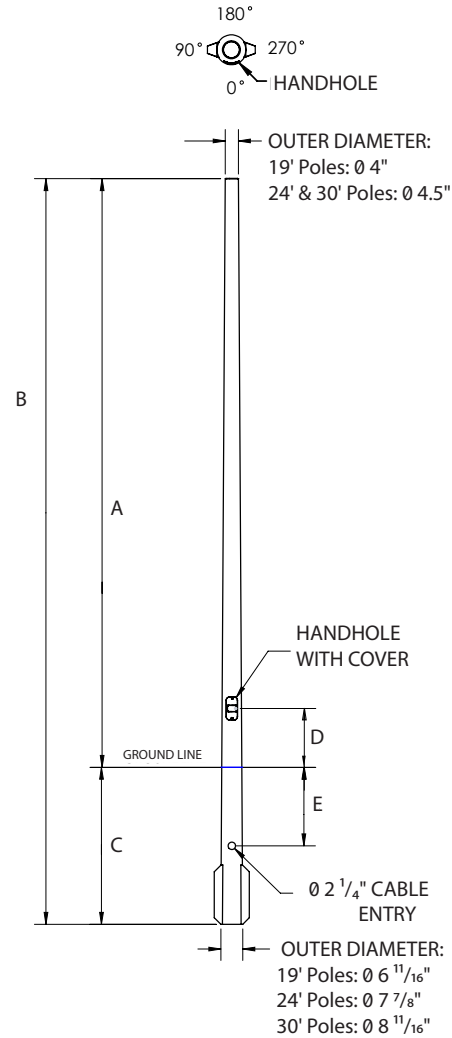
CD - Composite Tapered Direct Bury - Drilled
