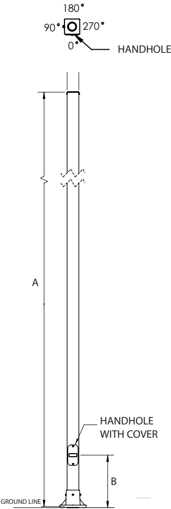
C - Composite Square w/Anchor Base- Drilled
