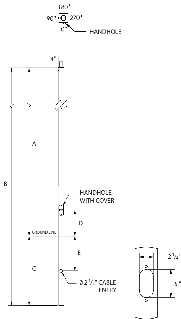
CD - Composite Square Direct Bury - Tenon
