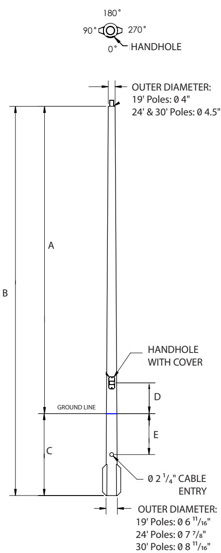
CD - Composite Tapered Direct Bury - Tenon
