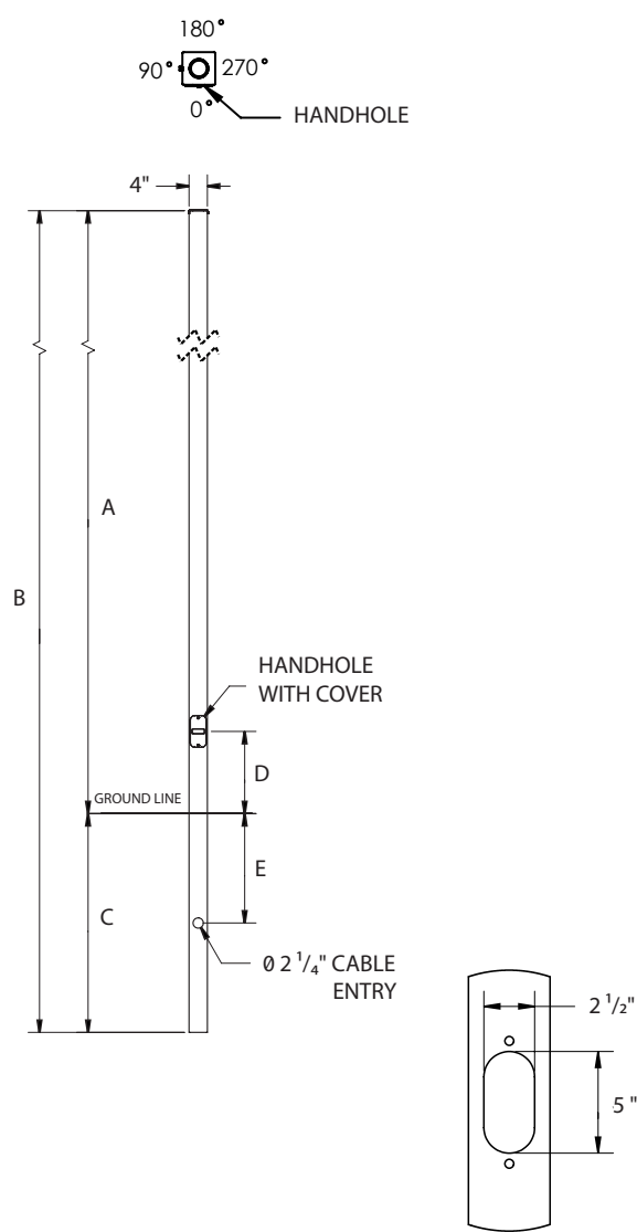
CD - Composite Square Direct Bury - Drilled
