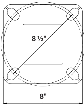
Poles with 4" shaft:
