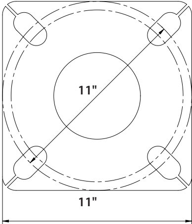
Flange dimensions:
