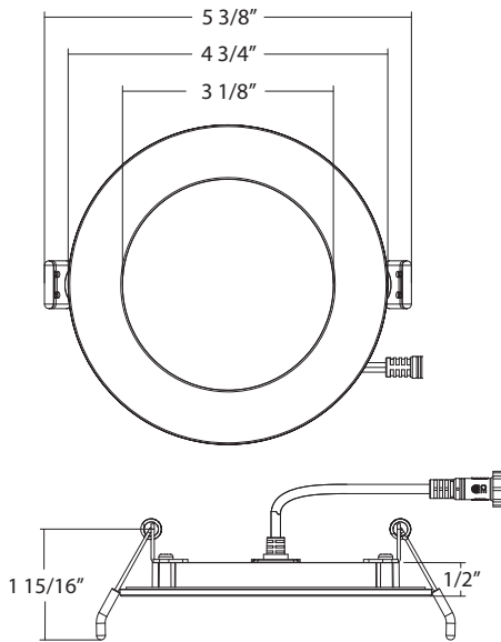
4" Smooth, Round
