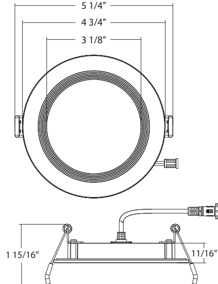
4" Baffle, Round
