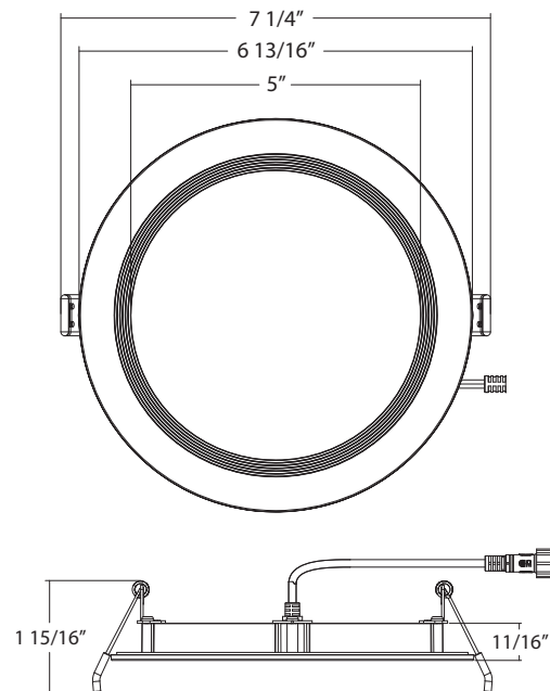
6" Baffle, Round
