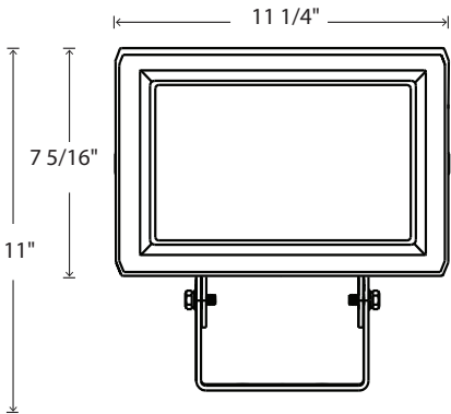
Trunnion Mount
