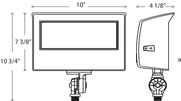
Knuckle Mount
