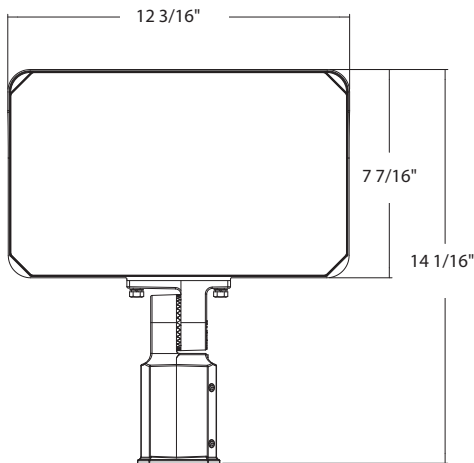
Slipfitter Mount
