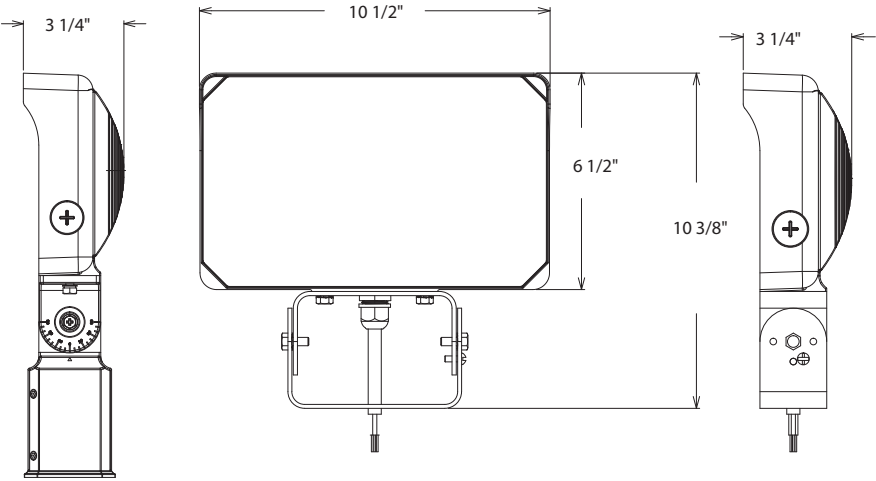
Trunnion Mount
