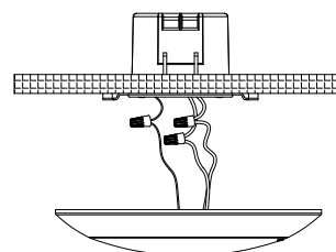
Mounting Bracket
