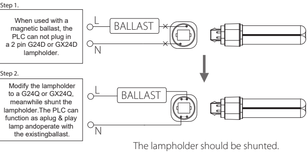
Fig.3- Magnetic ballast fixture wiring modification
