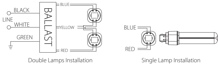
Fig.2- Electronic ballast fixture wiring
