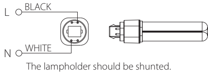
Fig.1- New fixture without ballast wiring
