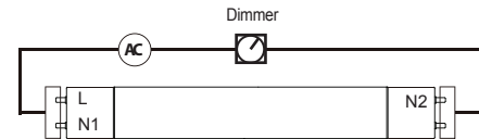
Fig:2 -Single-lamp with shunted lampholder
