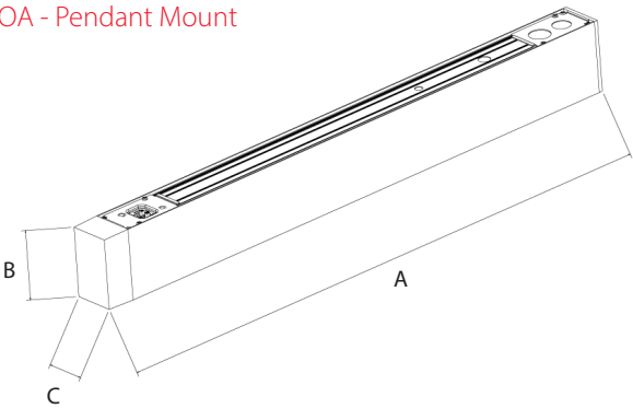
DIMENSIONS (PENDANT MOUNT MODELS)
