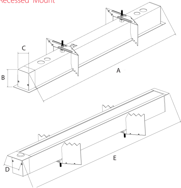
BOA - Recessed Mount
