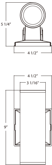
3" Cylinder - Standard & RGB Weight: 2.67lbs
