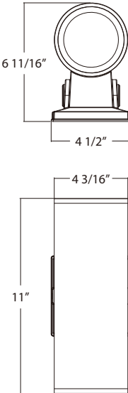
4" Cylinder - Standard & RGB Weight: 4.10lbs
