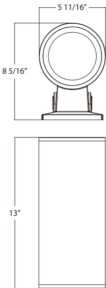
6" Cylinder - Standard & RGB Weight: 6.35lbs
