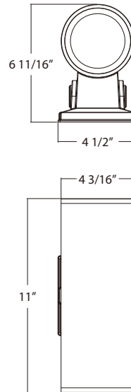
4" Cylinder - Standard & RGB Weight: 4.10lbs
