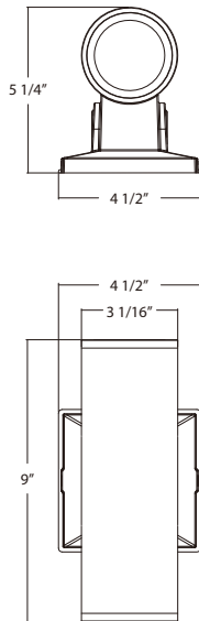
3" Cylinder - Standard & RGB Weight: 2.67lbs
