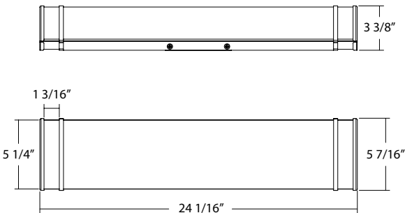
ENCT-24BN Weight: 2.87 lbs
