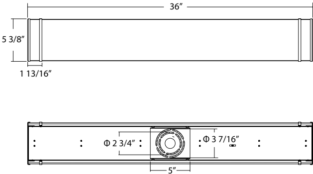
ENCT-36BN Weight: 3.48 lbs
