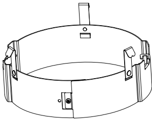
6" Band with Friction clips RFLED-RETROBAND For use with 6" housings without torsion spring receivers with internal diameter 165.1-171.45mm
