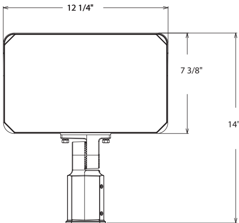
Slipfitter Mount
