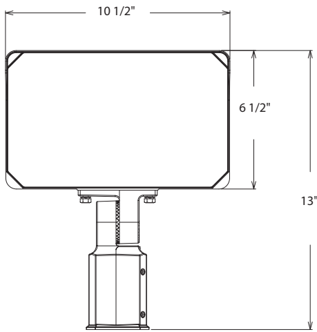
Slipfitter Mount
