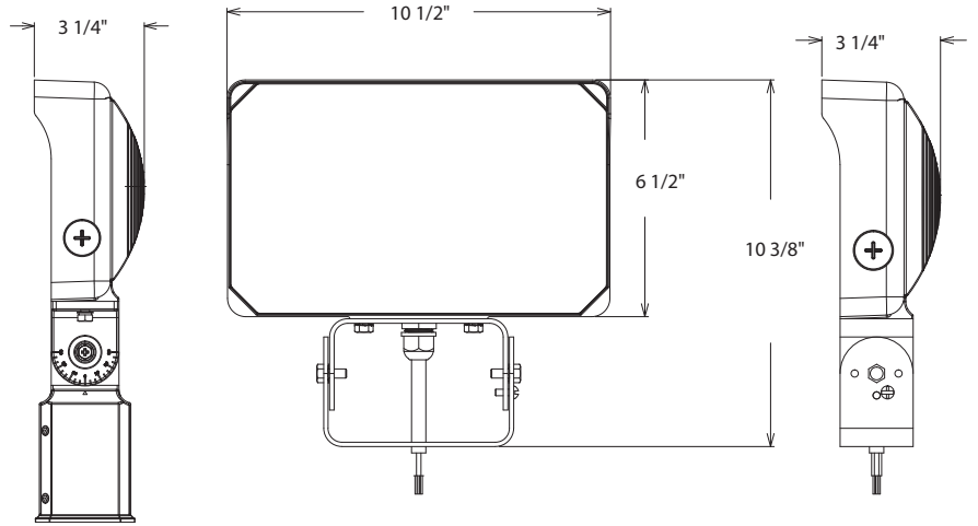
Trunnion Mount
