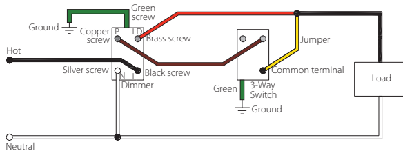
Wiring Scheme 3 (dimmer line side)
