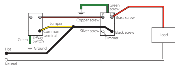
Wiring Scheme 6 (dimmer load side)
